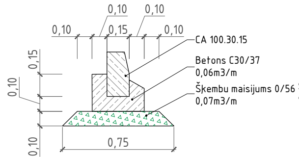
CA 100.30.15 M 1:25
